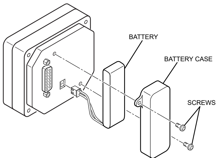
Figure 5.1, Battery Replacement
