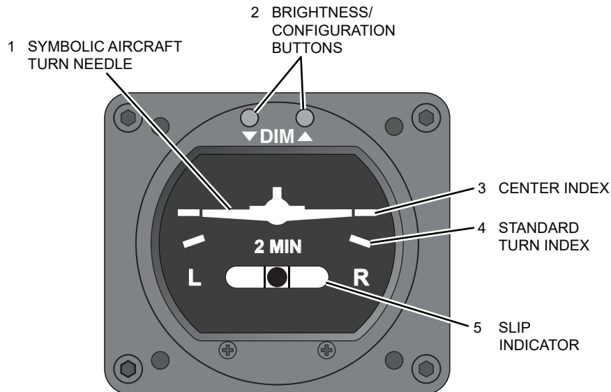
Figure 1.2, Typical Display Features - Turn Coordinator
